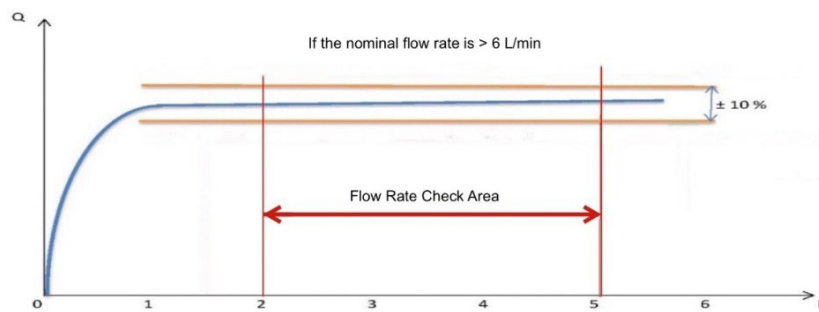
Figure 5: Verification of nominal flow rate of aerators
