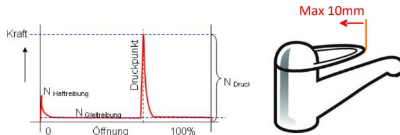
Figure 10: From left to right: graph Force/opening; point of measurement
