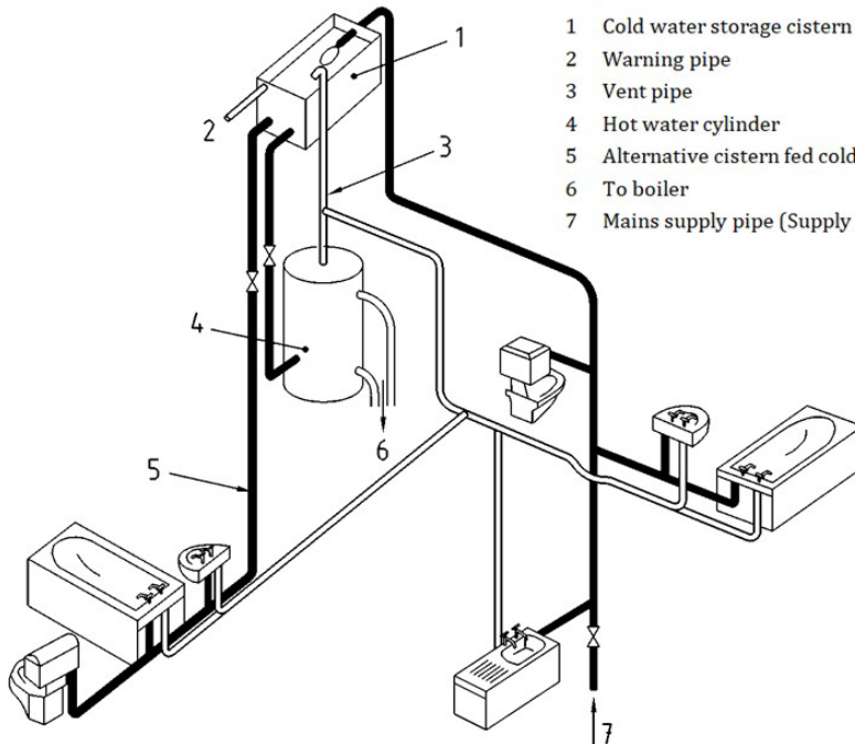
Figure 3: Type 2 supply system
